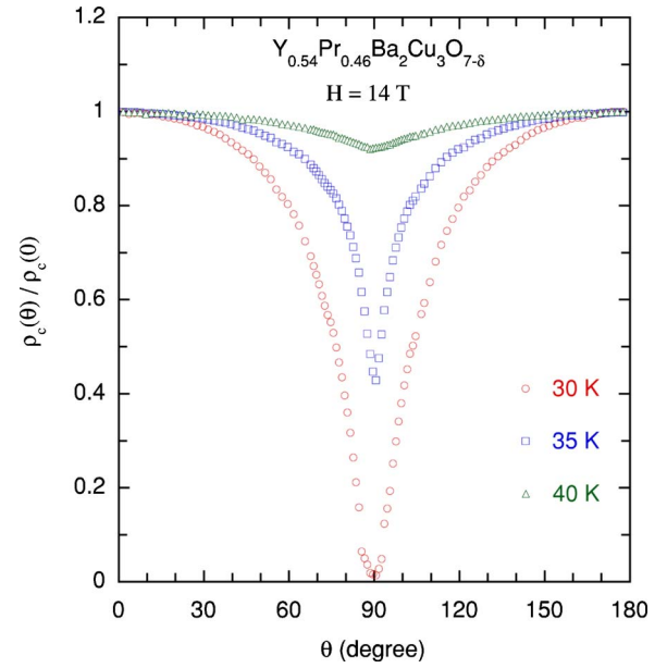
FIG. 2. (Color online) Angular \theta dependence of normalized out-of-plane resistivity \rho(\theta)/\rho(0) of an \text{Y}_{0.54}\text{Pr}_{0.46}\text{Ba}_2\text{Cu}_3\text{O}_{7-\delta} single crystal, measured at 30, 35, and 40 K and 14 T.
