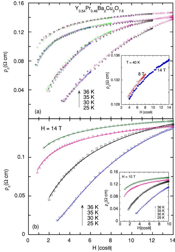
FIG. 3. (Color online) (a) Plot of the out-of-plane resistivity \rho_c vs H|\cos\theta of an \text{Y}_{0.54}\text{Pr}_{0.46}\text{Ba}_2\text{Cu}_3\text{O}_{7-\delta} single crystal, measured at 25, 30, 35, and 36 K and 6 T (open circles), 8 T (diamonds), 10 T (triangles), 12 T (inverted triangles), and 14 T (open squares). Inset: Plot of \rho_c(H|\cos\theta) measured at 40 K. (b) and its inset: Same plot of the data measured at 14 and 10 T, respectively. The solid lines are fits of the data with Eq. (7).
