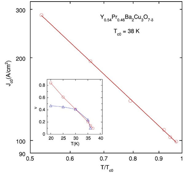
FIG. 4. (Color online) Josephson critical current density J_{c0} , calculated with the fitting parameters obtained by fitting the angular magnetoresistivity, vs reduced temperature T/T_{c0} . The solid line is a power law fit. Inset: Temperature T dependence of exponent \nu (empty circles) obtained by fitting the magnetoresistivity data. The theoretical \nu(T) dependence is calculated with the T dependence of the penetration depth \lambda_{ab}(T) given by the BCS theory and taking as the critical temperature T_{c0} = 38 K.
