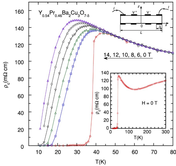
FIG. 1. (Color online) Temperature ( T ) dependence of out-of-plane resistivity \rho_c of an \text{Y}_{0.54}\text{Pr}_{0.46}\text{Ba}_2\text{Cu}_3\text{O}_{7-\delta} single crystal, measured in an applied magnetic field of 0, 6, 8, 10, 12, and 14 T and for T \leq 80 K. Insets: (top) Sketch of sample geometry and lead configuration; (bottom) zero-field \rho_c(T) shown over the whole measured T range. The solid lines are guides to the eye.
